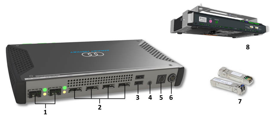
DXZ4-M rear view. 1 Network connections. 2 DisplayPort sockets. 3 USB ports. 4 Audio socket. 5 Feature connector. 6 DC inlet. 7 SFP modules. 8 Under-desk bracket (optional).
