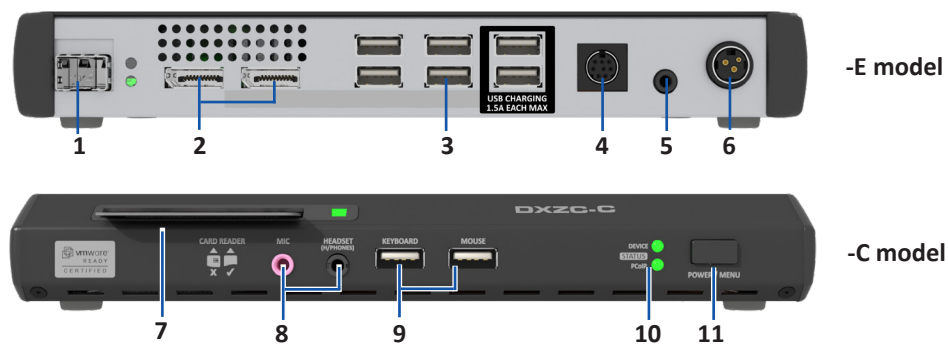
1 Network port. 2 DisplayPort connectors. 3 USB ports (two for high charge-current devices). 4 Feature connector socket. 5 Line-level audio output. 6 DC power inlet. 7 Card reader. 8 Mic and headset sockets. 9 Easy access USB. 10 LED indicators. 11 Power/Menu switch.
